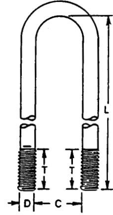
U-Bolt - Round Bend (D x L x C x T)
