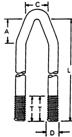
U-Bolt - Angle Bend (D x L x C x A x T)
