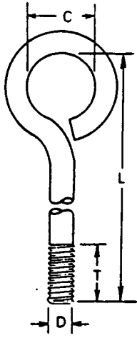
Eye Bolt - Closed (D x L x C x T)
