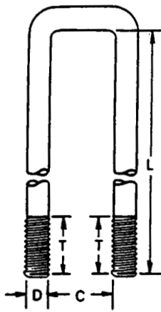
U-Bolt - Square Bend (D x L x C x T)
