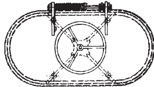
#215 Spring Balanced Oval Quick Acting Hatch
